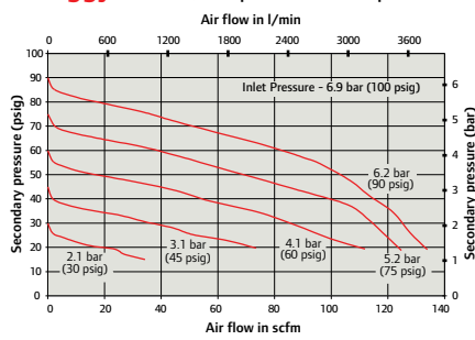
Piggyback 3/8" pressure drop test
